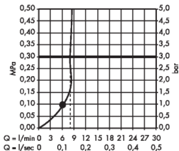
Crometta 85 1jet 28606000
